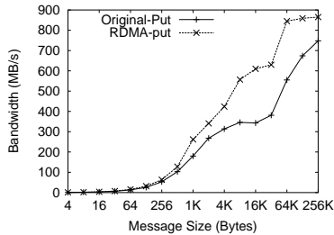
Figure 7. MPI_Put Bandwidth
