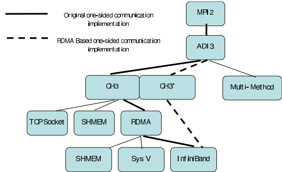
Figure 3. Design Architecture
