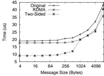
Figure 6. Bi-Directional Latency
