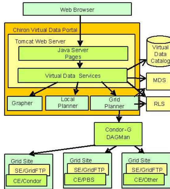
Figure 1. Chiron System Achitecture
