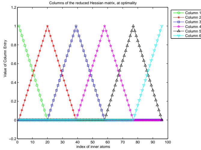
Figure 1: Columns of L_R .
