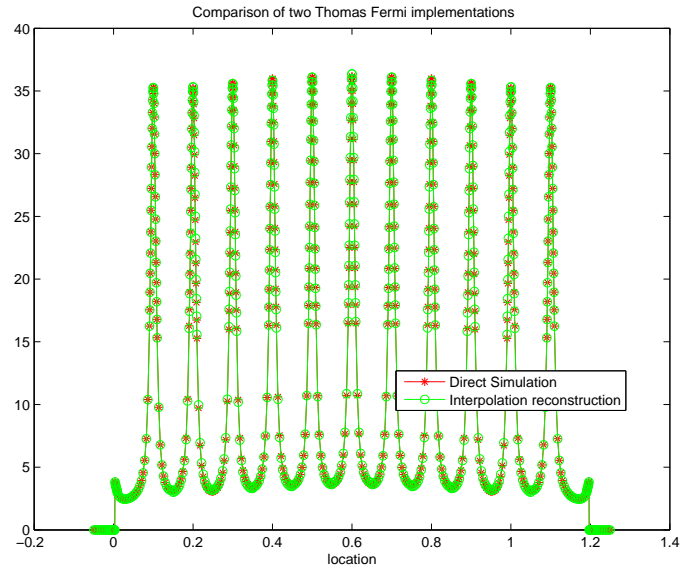
Figure 4: Solution to (O) and (RO) problems.
