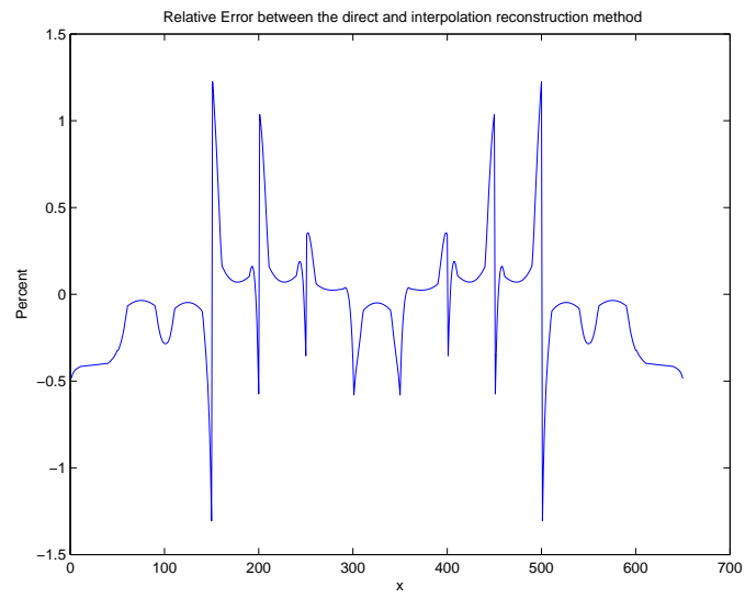
Figure 5: Point-to-point relative error between (O) and (RE).
