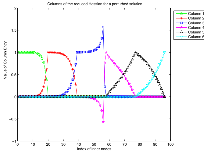
Figure 2: Columns of L_R , perturbed configuration.
