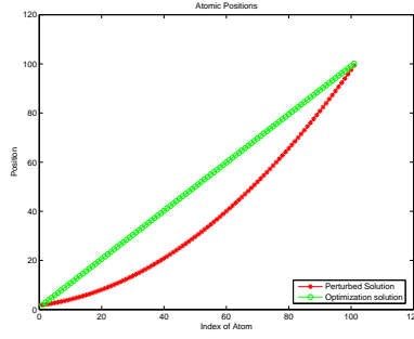
Figure 3: Positions of original and perturbed solutions.
