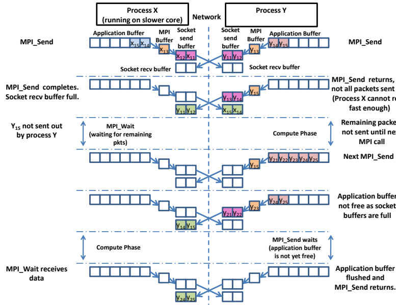
Figure 10: LAMMPS Timeline
