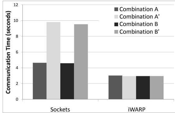
Figure 12: LAMMPS Performance
