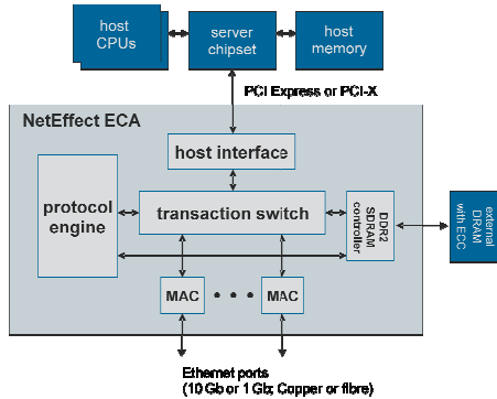
Figure 1: NetEffect iWARP NIC Architecture
