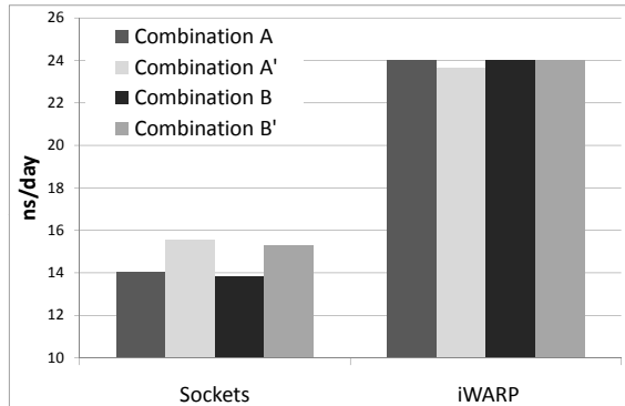
Figure 8: GROMACS LZM Protein System Application
