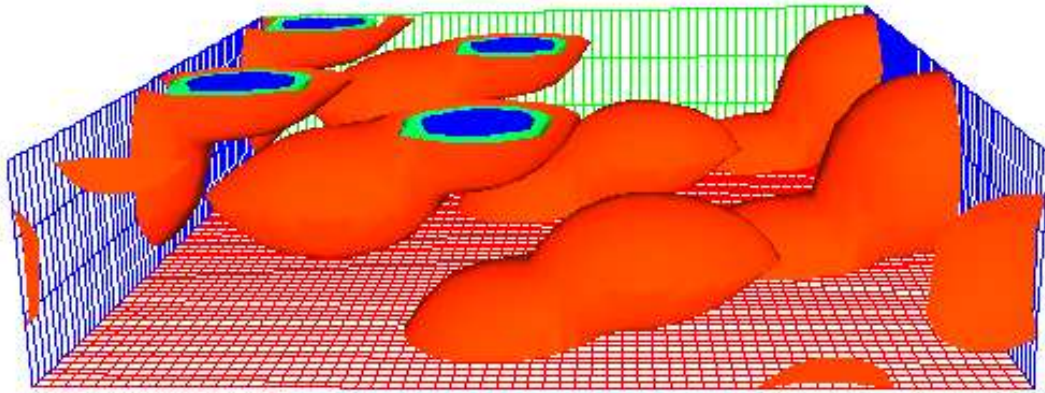
FIG. 9. View looking down on the layers of the vortex structure in the layered three-dimensional model. Pictured are isosurfaces of the order parameter magnitude. Recall that the order parameter is defined only within the superconducting sheets.
