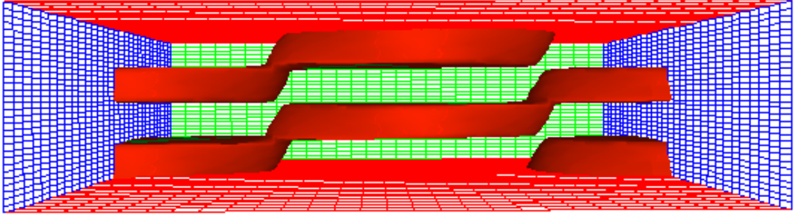
FIG. 8. View parallel to the layers of the vortex structure in the layered three-dimensional model. Pictured are isosurfaces of the magnetic field magnitude as the vortices cross superconducting layers.
