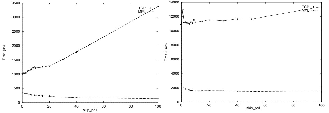
Figure 6: One-way message latency as a function of skip_poll for a microbenchmark in which two ping-pong programs run concurrently over MPL and TCP, as described in the text. The graph on the left is for zero-length messages, and the graph on the right is for 10 kilobyte messages.
