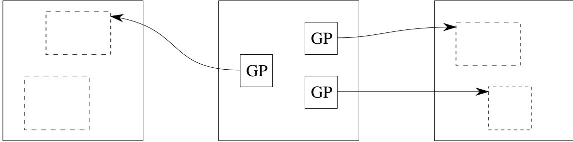
Figure 1: The global pointer and its role in communication. The figure shows three address spaces; three global pointers in address space 1 reference objects in address spaces 0 and 2.
