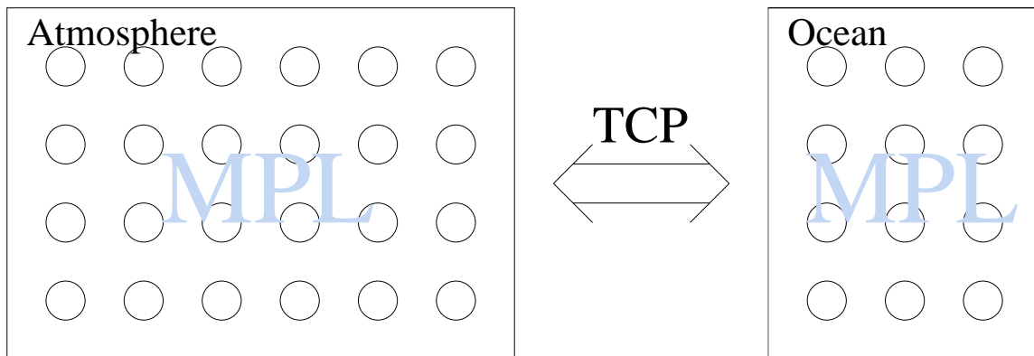
Figure 7: The Argonne/Wisconsin coupled ocean/atmosphere model in the configuration used for our multimethod communication experiments, showing the two IBM SP partitions.
