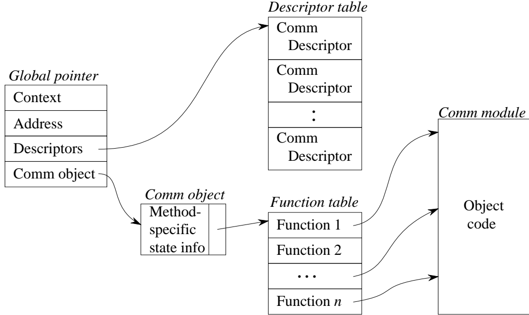
Figure 2: Nexus data structures used to support multimethod communication. The figure shows the global pointer, communication descriptor table, communication object, function table, and communication module. The data structures are explained in the text.
