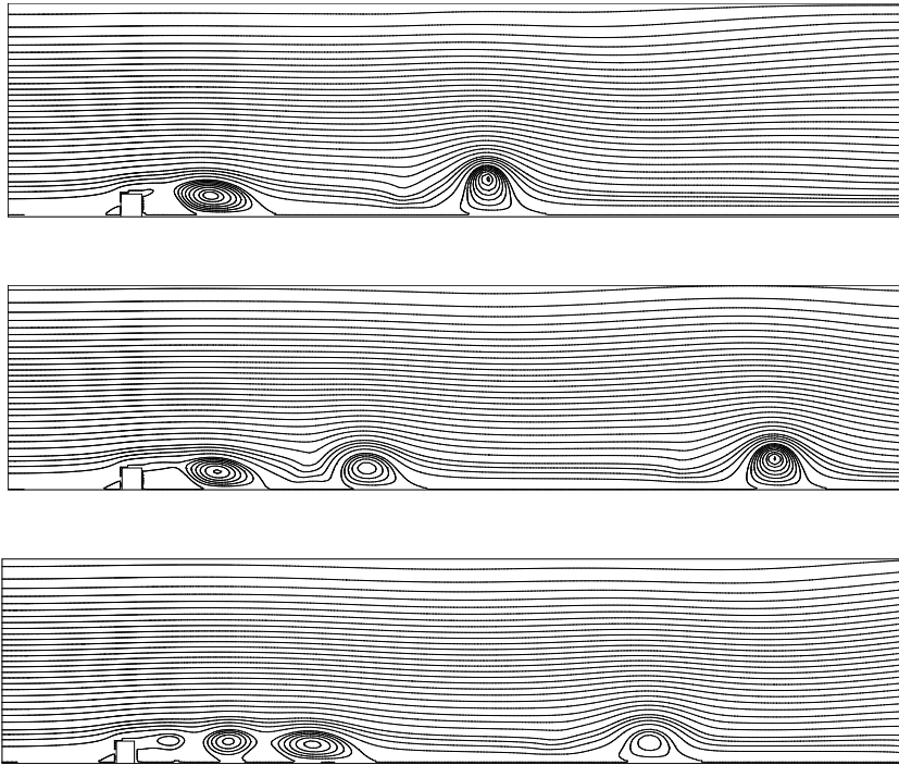
FIG. 3. Example 3, streamlines for t = 50, 75, 100 .
