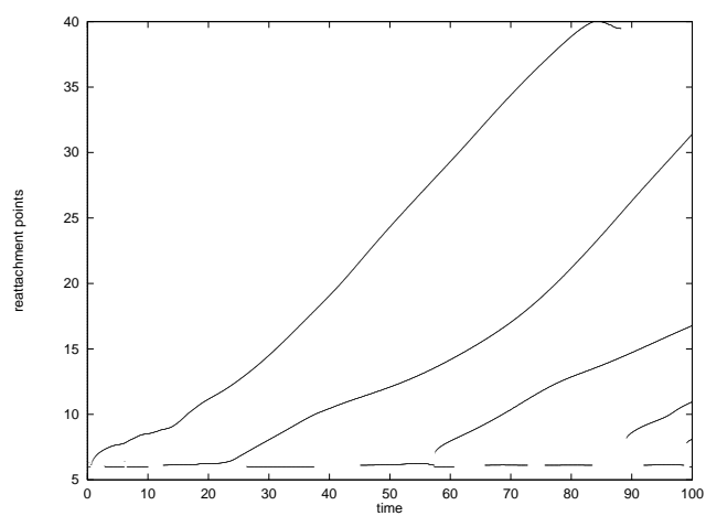
FIG. 2. Example 3, reattachment points.
