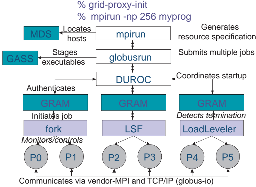
FIG. 1 Schematic of the MPICH-G2 startup, showing the various Globus Toolkit components used to hide and manage heterogeneity. “Fork,” “LSF,” and “LoadLeveler” are different local schedulers.
